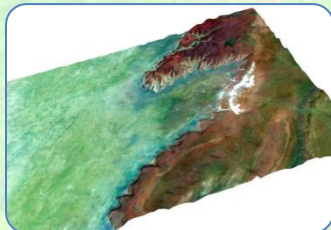
Satellite imagery
